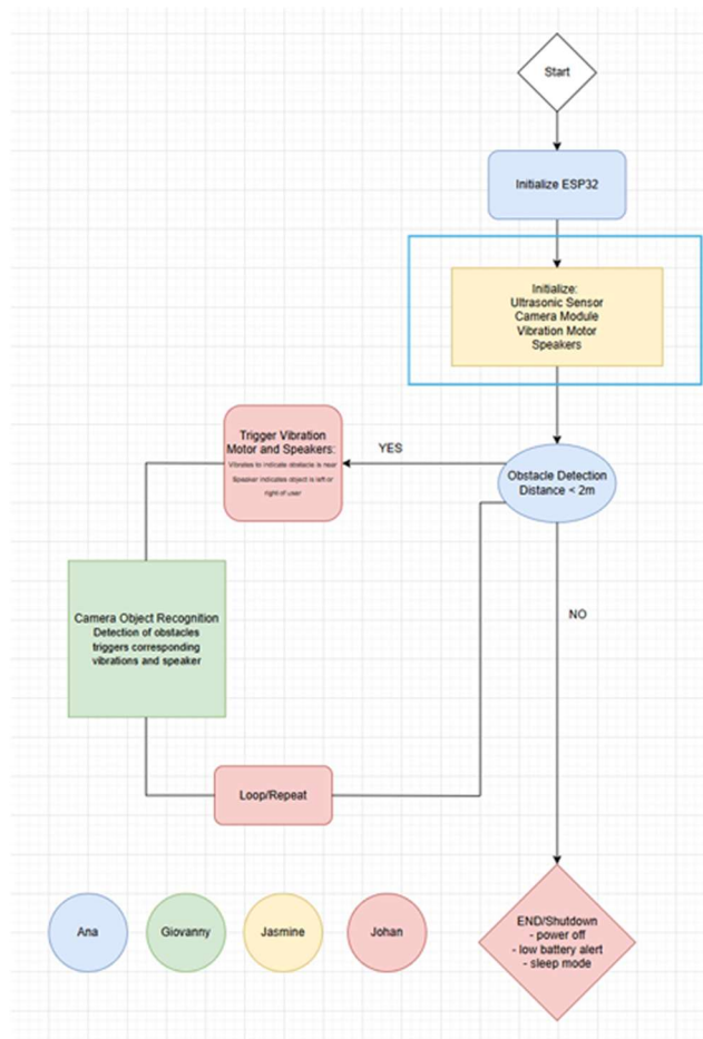
Fig 1. System Flowchart
