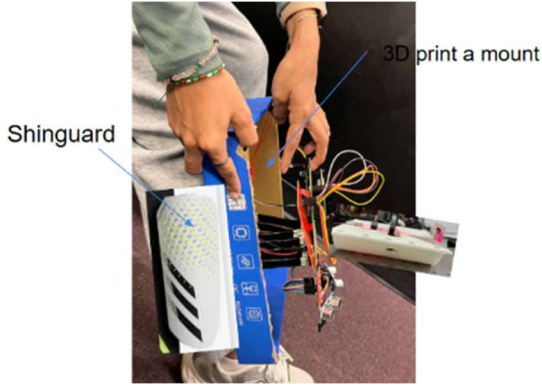
Fig. 7. SightSense Design
